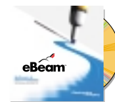
eBeam software
